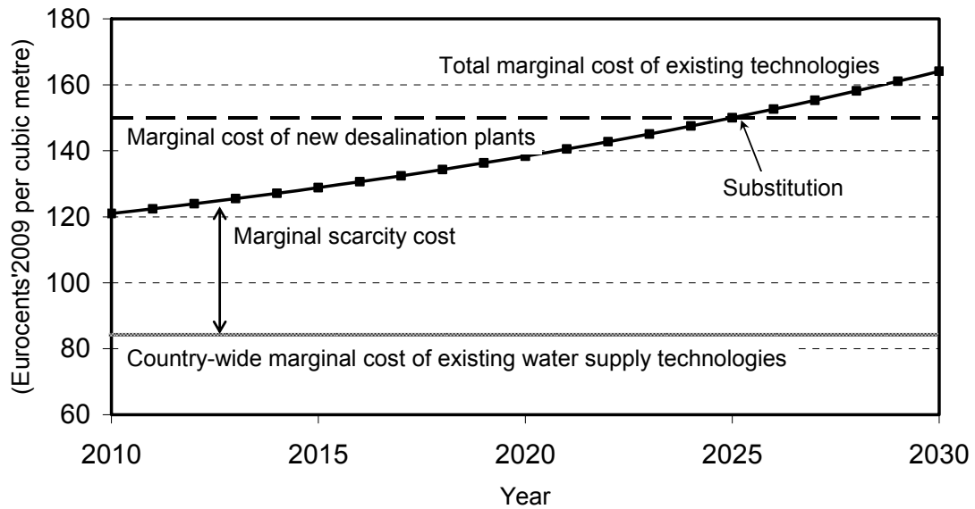
Figure 2: Evolution of marginal water supply costs in the period 2010–2030 according to results of scenario 2; from 2025 onwards existing water supply options are substituted by new desalination plants.
